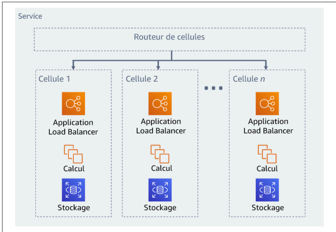
Figure 11 : Architecture cellulaire
