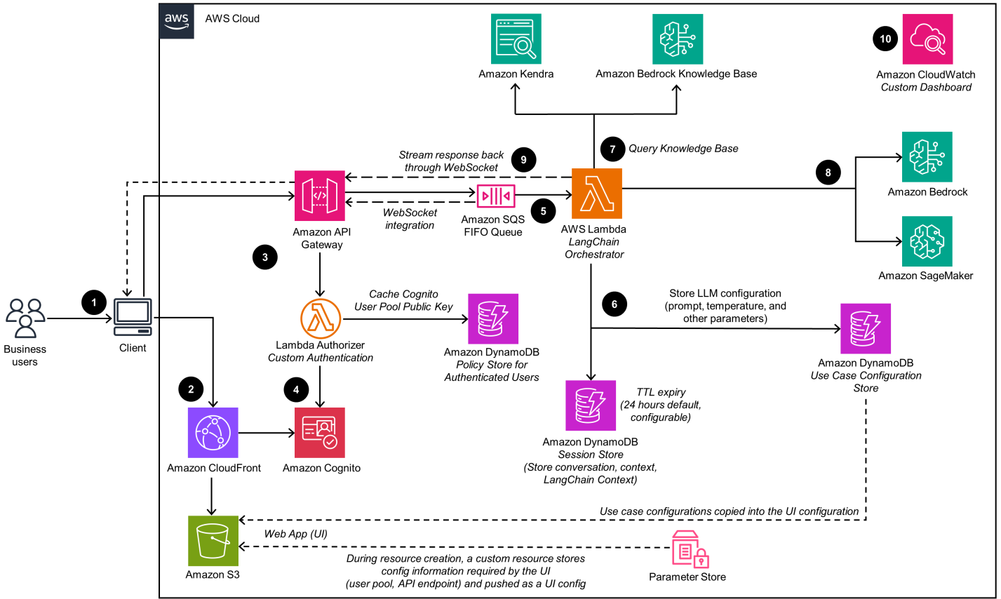
Text use case architecture (when deployed with VPC option disabled)
