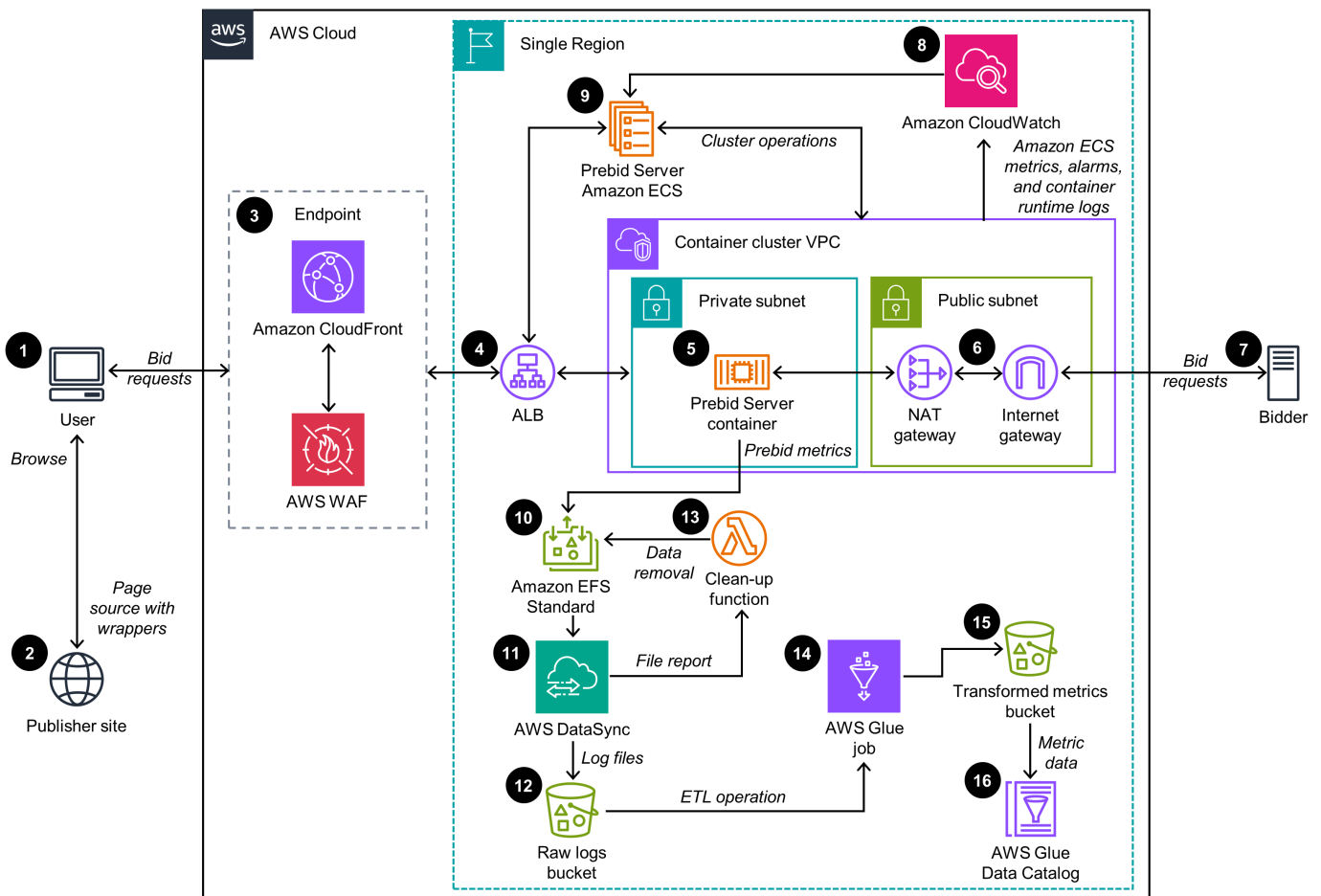
Prebid Server Deployment on AWS architecture
