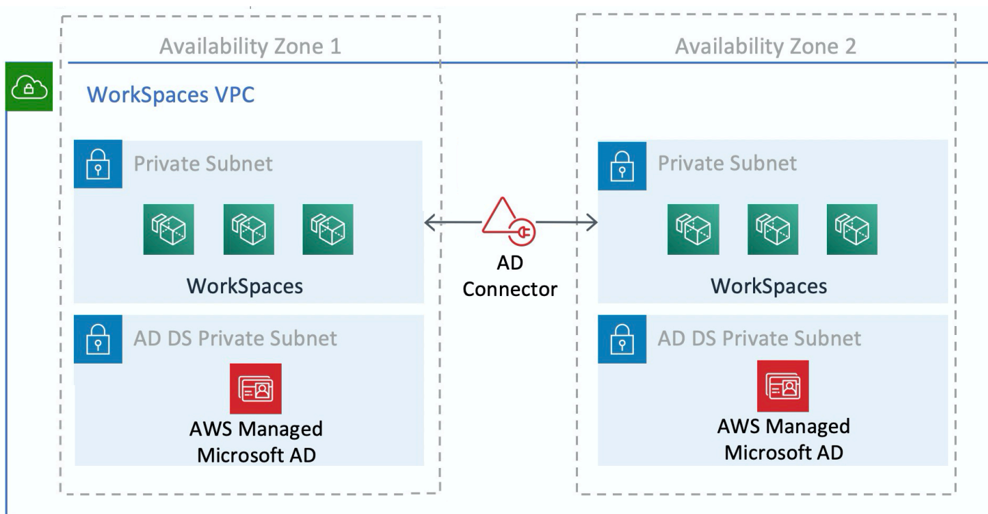
Figure 13: AD DS network separation
