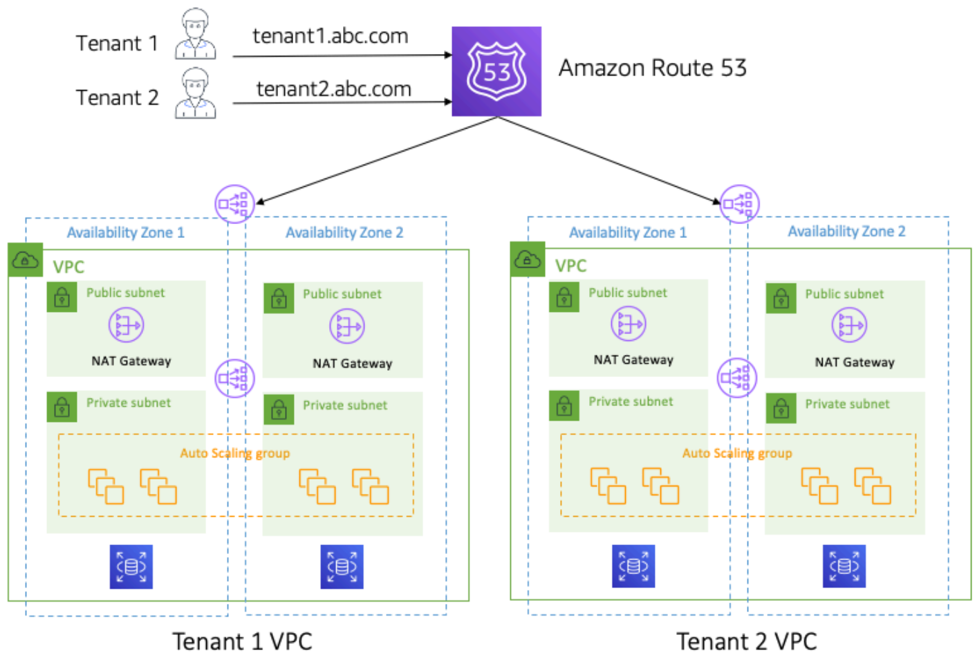
Figure 7: Full stack (silo) isolation
