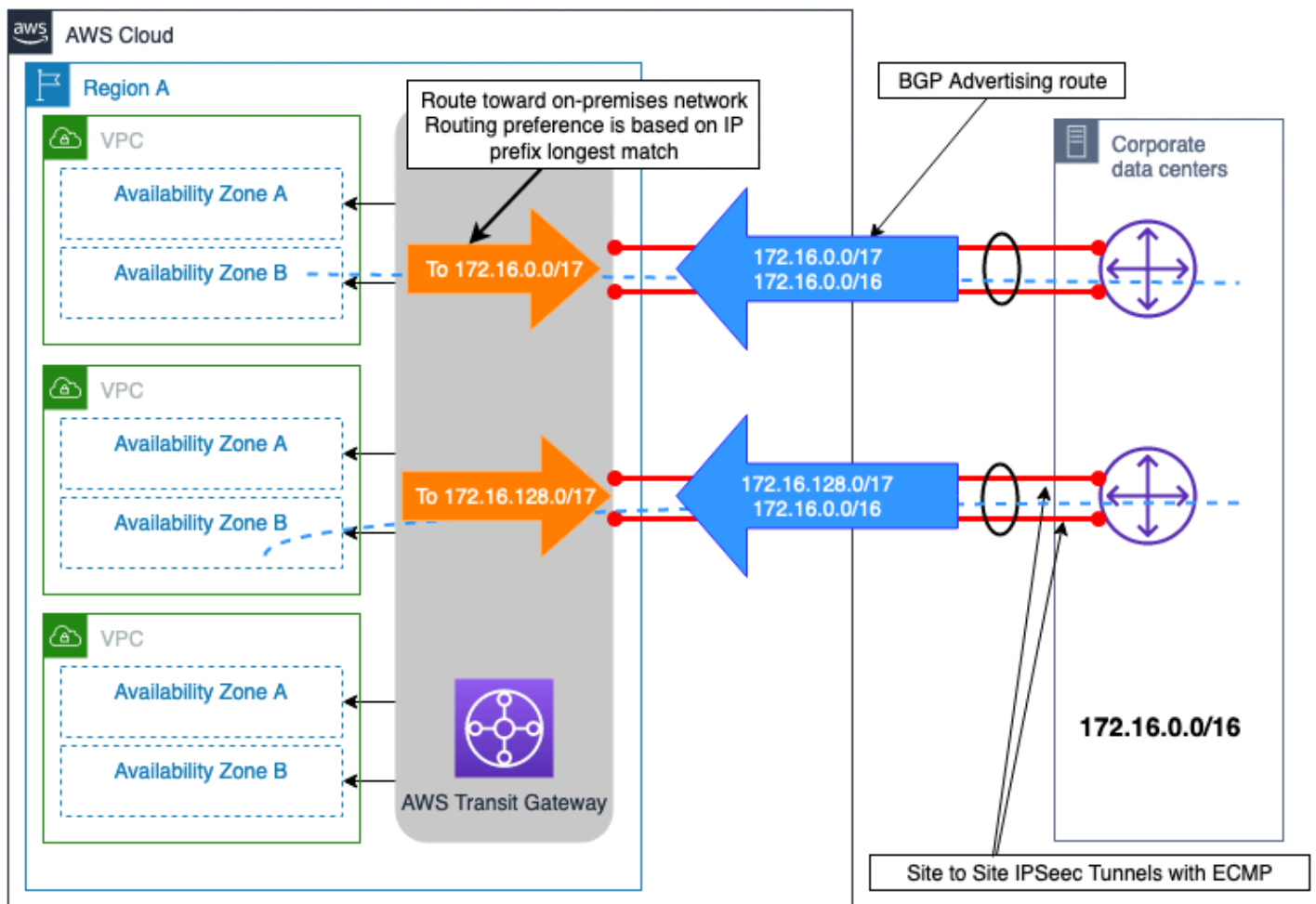
Figure 10 – Dual Site-to-Site VPN connections with more specific routes example
